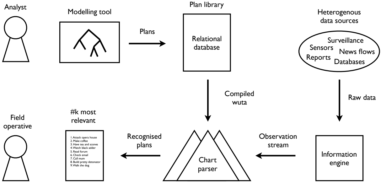
Figure 3: The user works with a modeling tool to create and edit plans. The plans are stored in a plan library and compiled upon demand into a wuta. The wuta can be used to parse observations streams and produce a list of the k plans that are most likely to be active in a given moment.
