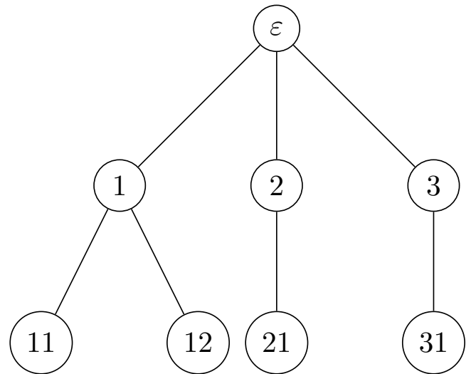
Figure 2: A realisation of the plan tree in Figure 1.
