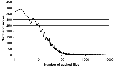
Figure 6: Distribution of the number of files per node for the eDonkey file trace [12].
