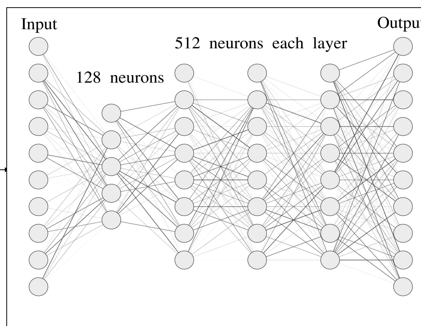
Figure 1. Our neural network architecture
