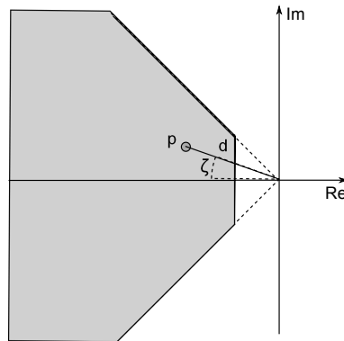
Figure 1: A pole p with distance d to the origin and angle \zeta . The shaded area shows where it is usually safe to place poles in continuous time systems.
