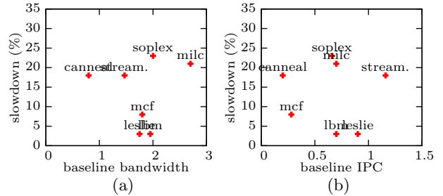
Figure 8: Correlation of slowdown with baseline bandwidth (a) and IPC (b) when the total bandwidth is 90% of the saturation bandwidth.
