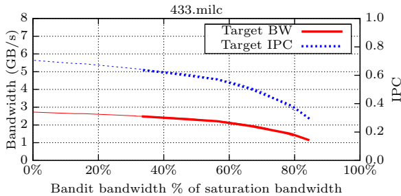
Figure 6: Bandit bandwidth as percentage of the saturation bandwidth. Data captured with a random-access bandit (thin lines) and a sequential-access bandit (thick lines).
